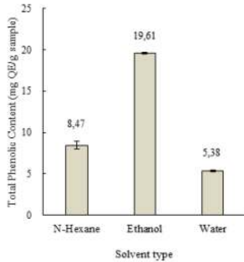
Figure 2. Total Phenolic Content of A. decurrens gum extract from multilevel extraction using 3 different solvents (means of 3 replications)
