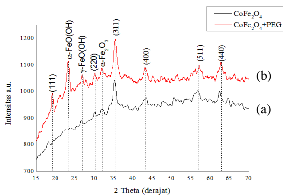
Gambar 1. Pola spektrum XRD; (a) CoFe 2 O 4 ; (b) CoFe 2 O 4 +PEG-4000
