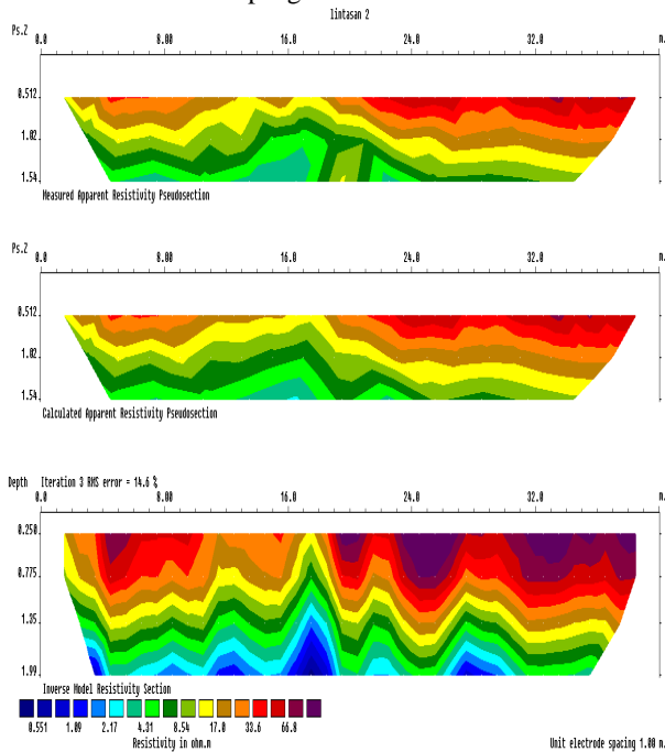
Gambar 2.2 Penampang resistivitas lintasan 2
