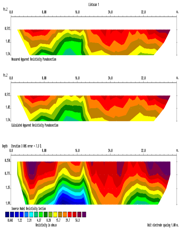
Gambar 2.1 Penampang resistivitas lintasan 1
