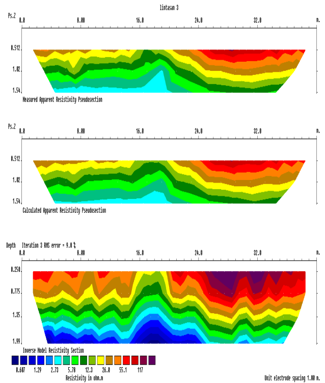
Gambar 2.3 Penampang resistivitas lintasan 3
