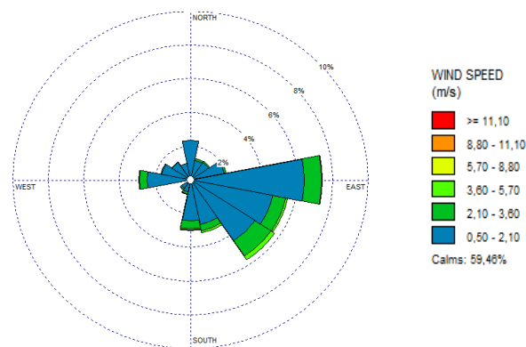
Figure 7. Regional Wind Rose Chart of 2019
