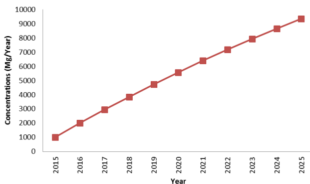
Figure 3. Graph of Methane Gas Formation Based on Pre-Processed Data Using the IPCC Method (Source : LandGEM, 2020)
