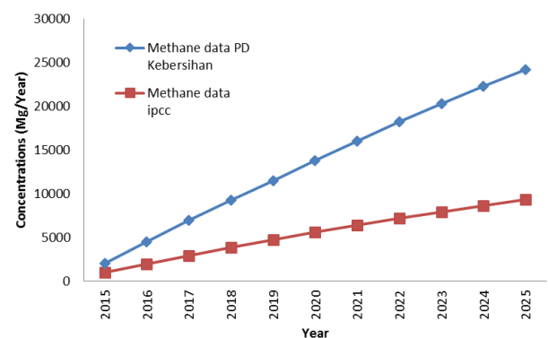
Figure 4. Comparison Graph of LandGEM Method Methane Emissions
