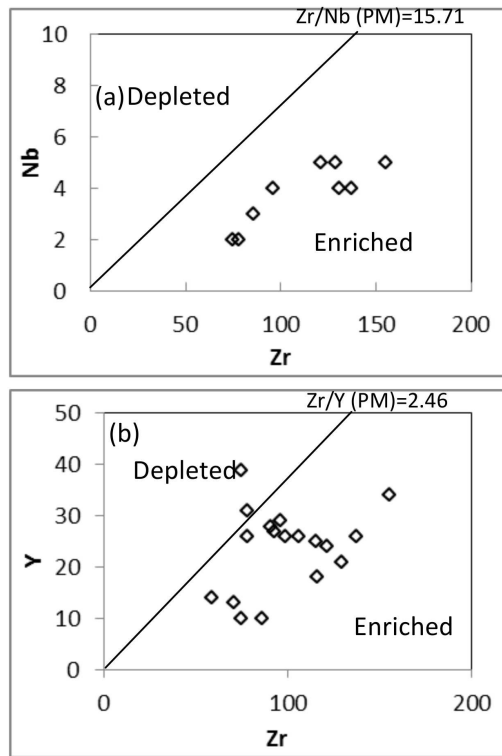
Figure 10: Plots of Zr versus (a) Nb and (b) Y for volcanic host rocks showing the less mobile nature of these elements and illustrating the sensitivity of these element ratios to source composition. Primordial mantle ratios after Sun and McDonough (1989).
