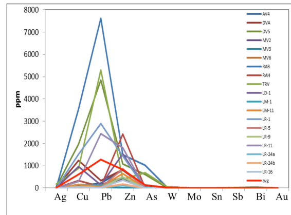
Figure 11: Ore-forming elements compositions of the host rocks.
