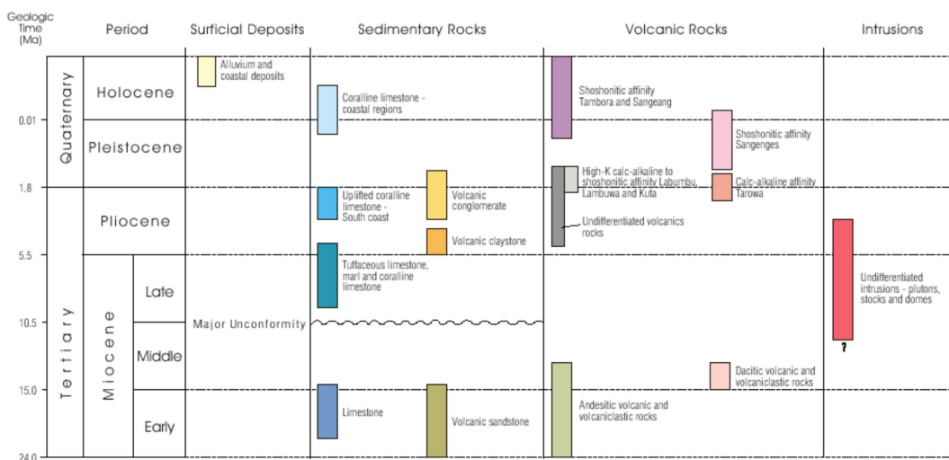
Figure 1: Simplified geologic map and chronology map units of Sumbawa island, Indonesia including Soripesa prospect area (Garwin, 2002).
