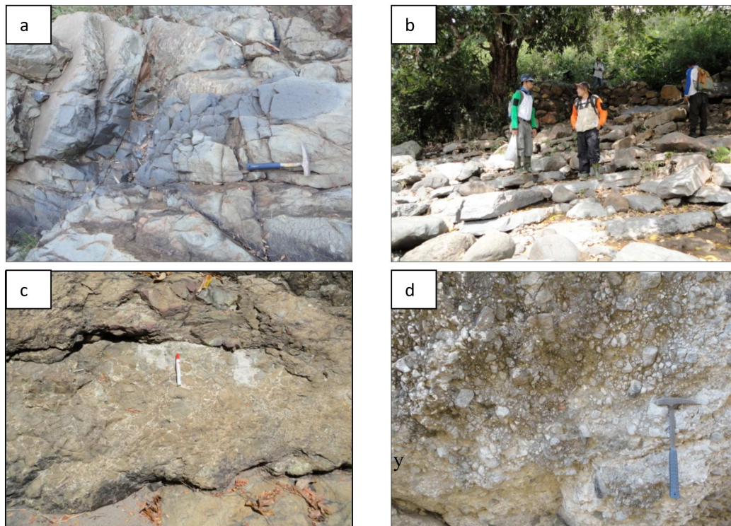
Figure 3: (a) Andesitic volcaniclastic rock (b) Fossiliferous limestones (c) Dacitic volcaniclastic rock (d) Quaternary agglomerate rocks.
