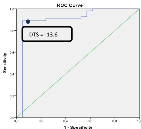
Figure 1.The ROC curve of DTS value to assess Syntax score
