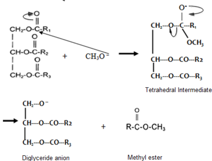
Fig 3. Reaction mechanism of catalyst to form biodiesel from waste cooking oil
