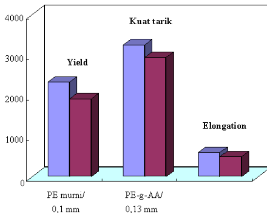
Gambar 7. Hasil analisis kuat tarik film PE dan film PE tergrafting asam akrilat 30%. Yield : ( ) PE, ( ) PE-g-AA 30% ; Kuat tarik : Yield : ( ) PE, ( ) PE-g-AA 30% ; Elongation : ( ) PE, ( ) PE-g-AA
