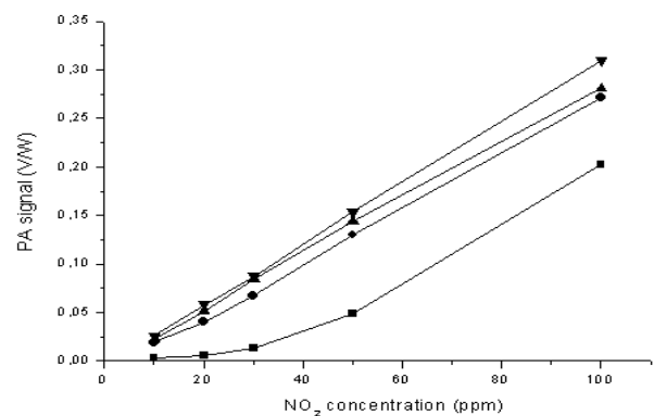
Figure 3. – Values of PA signal vs. NO 2 concentration in N 2 at different flow rates at a laser power of 42 mW. : 2 l/h; ? 10 l/h; ? 15 l/h; ? 20 l/h
