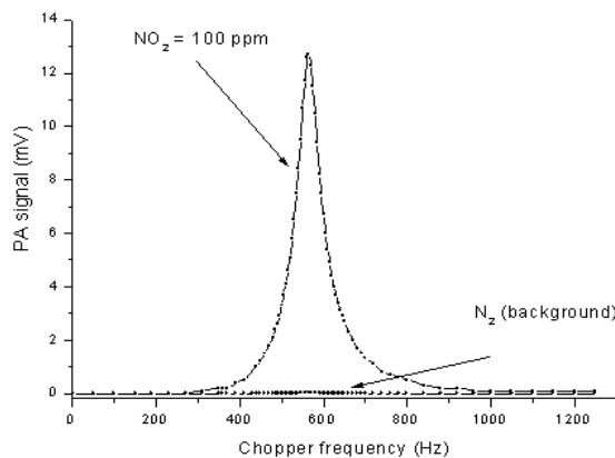
Figure 2- Resonance frequency of the PA cell
