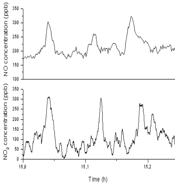
Figure 6. – Values for NO 2 and NO concentration from urban air around 3:00 PM June 15 th , 2006
