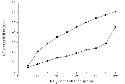
Figure 5 - NO vs. NO 2 concentration measured by the QCL and photoacoustic system, respectively. □ NO 2 in N 2 ; ○ NO 2 in air. The gas flow rate in the PA system is 15 l/h
