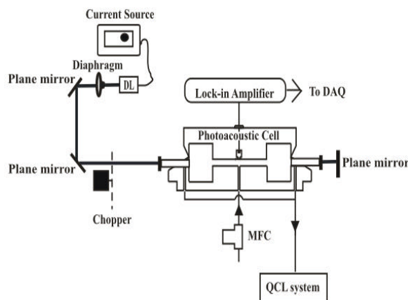
Figure 1. – Photoacoustic spectroscopy (PAS) system experimental setup. The laser beam from the diode laser (DL) is passed twice through the photoacoustic (PA) cell by using a plane mirror behind it. The gas output from PA cell goes to the QCL system. DL: Diode laser, MFC: mass flow controller, DAQ: data acquisition card, QCL: quantum cascade laser
