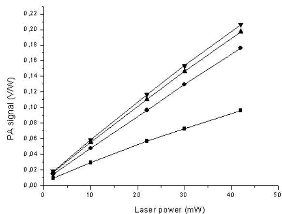
Figure 4. – Values for PA signal vs. laser power at different gas flow rates of the 100 ppm NO 2 concentration in N 2 . : 2 l/h; ? 10 l/h; ? 15 l/h; ? 20 l/h
